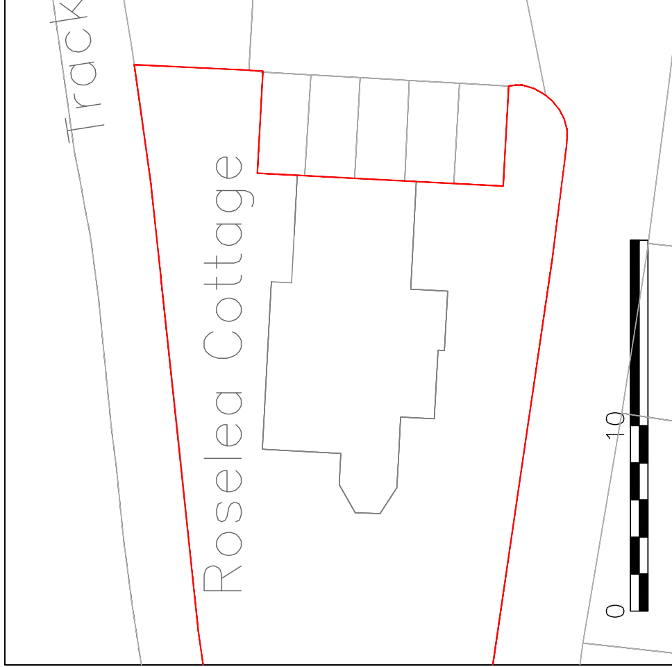
BLOCK PLAN 1:200
